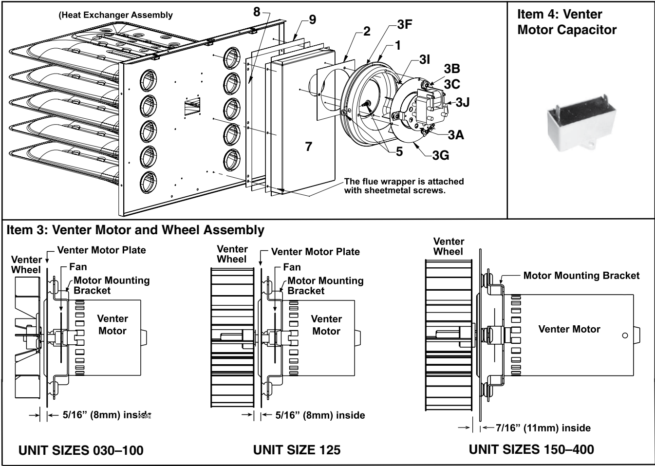
Figure 7. Venter and Flue Wrapper Components (Refer to Table 17 and Table 18 )
